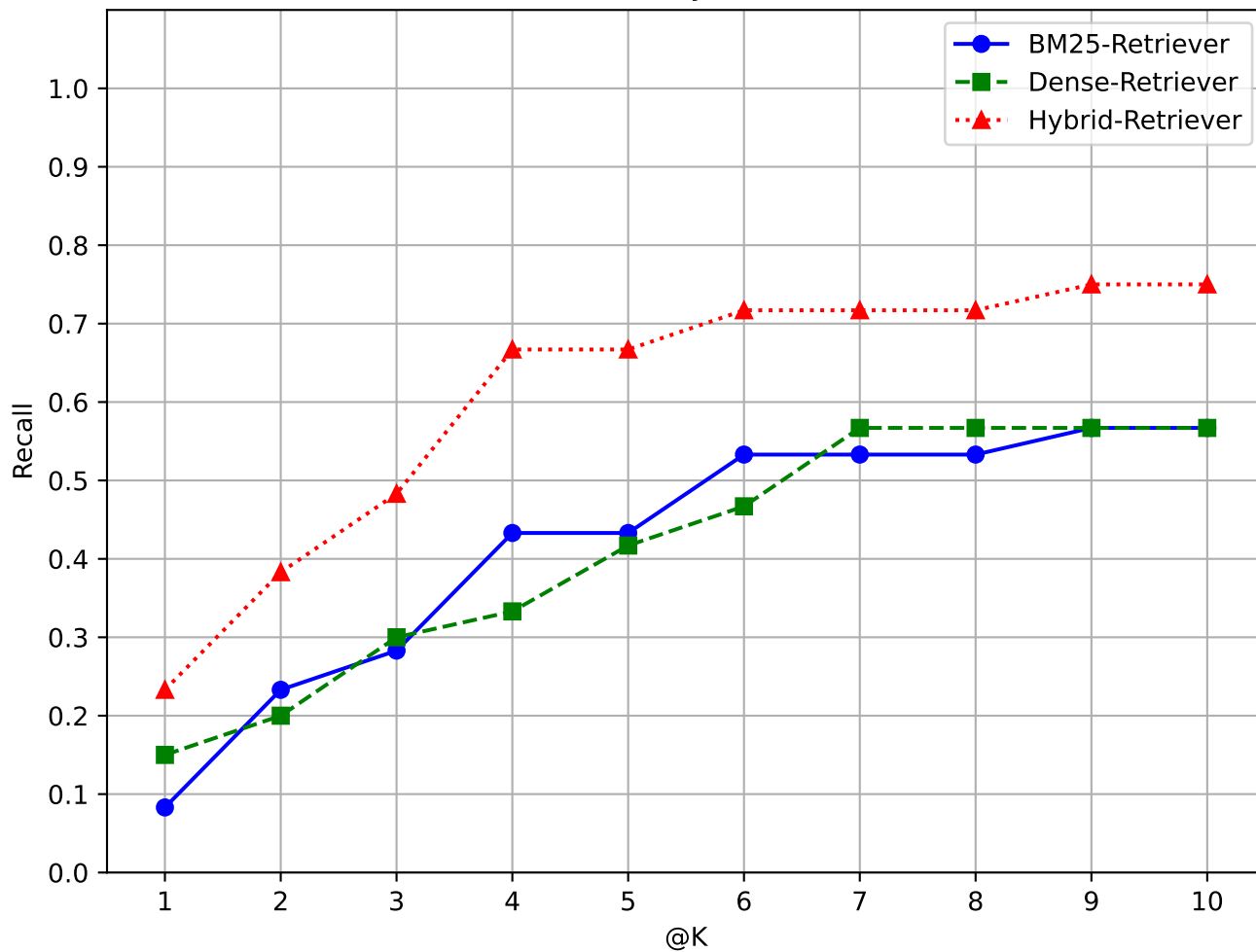
Query 29
